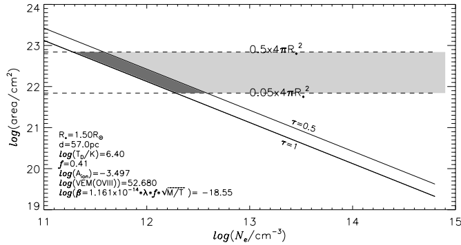
Fig. 4. Area vs. density N_e from the requirement optical depth \tau < 1 ; area values for surface filling factors are indicated.
