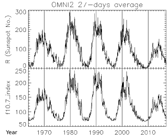
Figure 9. 27 day averages of: Upper panel: SIDC (new) sunspot number; lower panel: NRC F10.7-cm coronal radio flux (source: OMNI/NASA).
