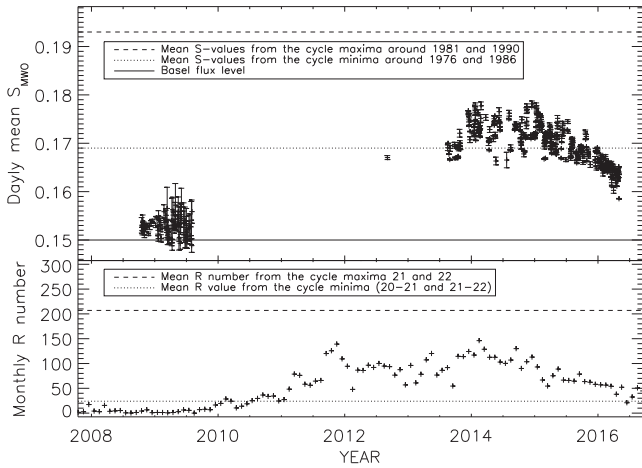
Figure 3. TIGRE’s Mount Wilson-calibrated S-index values of the 2008/2009 (last activity minimum) and 2013–2016 period (error bars refer to measurement uncertainties only; calibration errors may reach 0.004), in perspective with previous average minimum and maximum activity (lines; see Section 4.1) and SIDC monthly sunspot numbers (below). The chromospheric emission of cycle 24 is much lower than in previous cycles.
