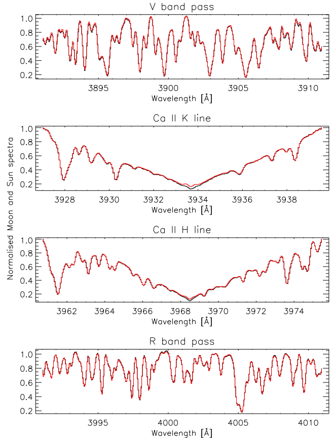
Figure 4. Comparison of a solar KPNO FTS spectrum (red; reduced to a spectral resolution of 20 000 for better comparability) and a TIGRE moon-light spectrum (black) in the spectral range relevant for the S-index measurements; see the text for details.
