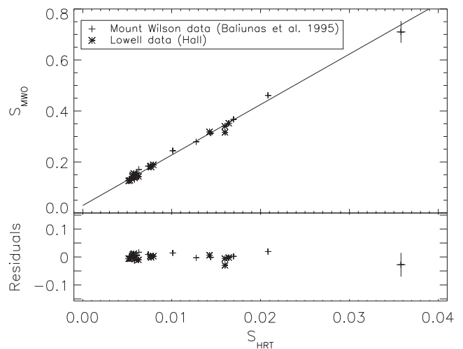
Figure 1. TIGRE S-index calibration for the observations taken in Hamburg in 2008/2009 (Mittag et al. 2011).
