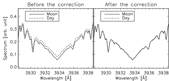
Figure 5. Moon and sky-scattered sunlight spectra before and after the scattering correction.
