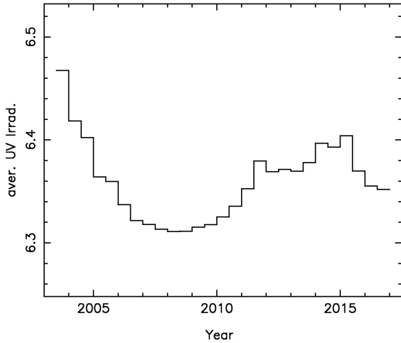
Figure 10. SOLSTICE/SORCE integrated spectral irradiance of the far-UV 200–280-nm window, relevant for stratospheric warming by photodissociation of molecules, averaged over periods of half a year between 2003 and 2016. The maximum of the present 24th cycle appears equally reduced as observed in TIGRE S-index time series calibrated to the Mount Wilson scale.
