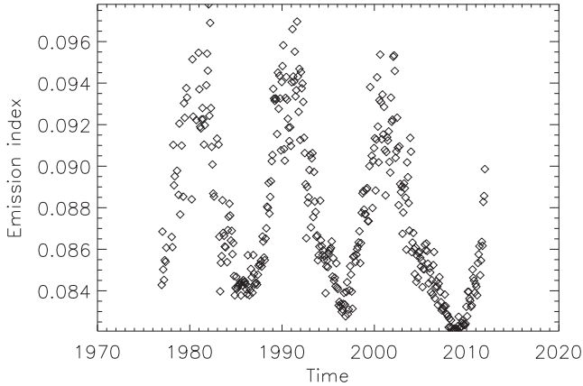
Figure 8. Monthly medians of the SOLIS-calibrated Ca II K 1-Å index time series of the NSO (source: data made available by Bertello et al. 2017).
