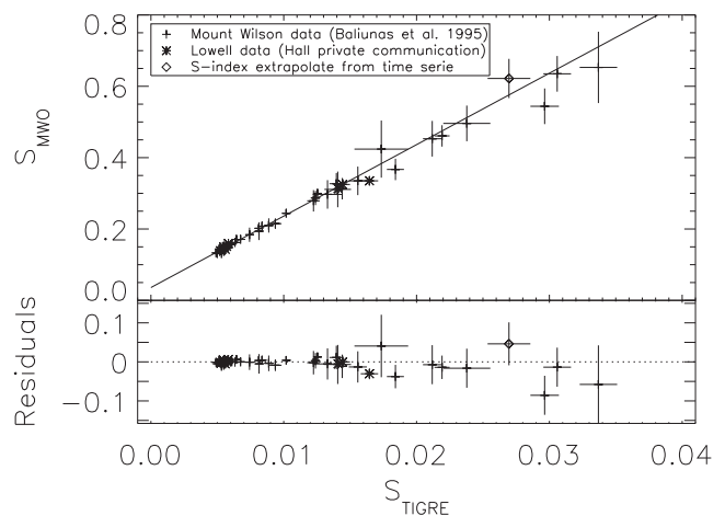
Figure 2. TIGRE S-index calibration for the La Luz data taken since 2013 (Mittag, Schmitt & Schröder 2016).
