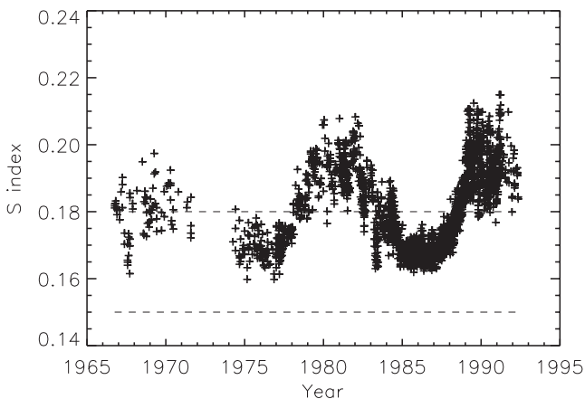
Figure 11. Historical solar Mount Wilson S-index values, covering the solar chromospheric activity from the 1960s to the 1990s, according to Baliunas et al. (1995). Horizontal lines mark extreme TIGRE S-index values of cycle 24.
