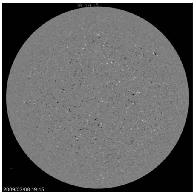
Figure 7. SOHO MDI magnetogram from 2009 March 8 ( https://sohodata.nascom.nasa.gov/cgi-bin/data_query ).
