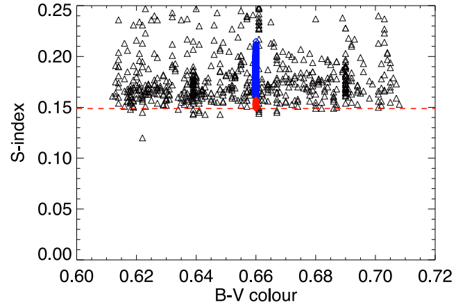
Figure 12. Stellar S-index values (triangles, taken from Mittag et al. 2013) in the colour range of 0.61–0.71, together with the solar S-index values shown in Fig. 11 (blue filled symbols over B-V = 0.66 ) and Fig. 3 (red symbols); the red dashed line marks the lowest TIGRE measured S-indices.
